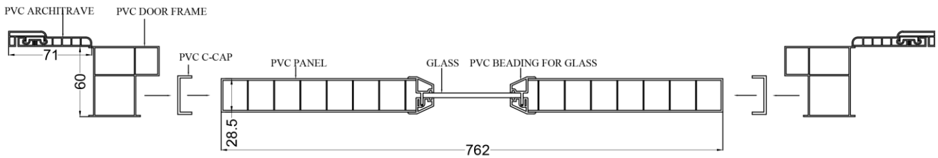
Line Diagram of Sections With Dimensions
